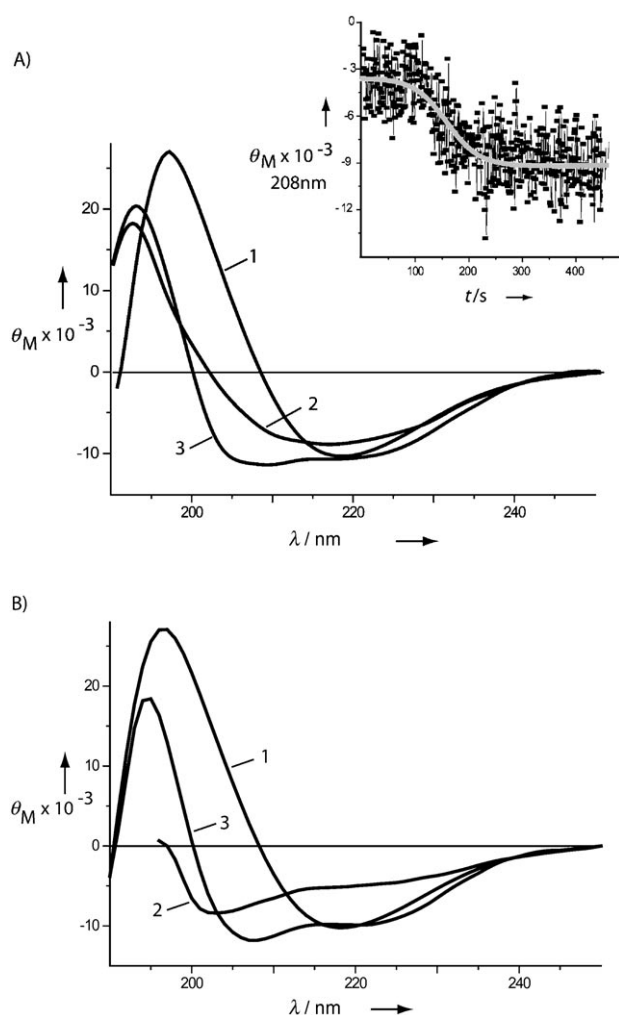
Figure 2. Conformational transitions of peptide I (see Figure 1) in the CD spectrum ( c = 5 \times 10^{-5} M, T = 25 °C): A) curve 1: pH 4.5 buffer ( S_{\text{off}} ); curve 2: pH 4.5 buffer/TFE 75:25 ( S_{\text{off}} ); curve 3: pH 7.0 buffer/TFE 75:25 ( S_{\text{on}} ). B) pH 4.5 buffer, curve 1: T = 25 °C ( S_{\text{off}} ); curve 2: T = 95 °C ( S_{\text{on}} ); curve 3: after cooling to T = 25 °C ( S_{\text{on}} ). Inset: the kinetics of the transformation from \beta -sheet ( S_{\text{off}} ) to \alpha -helix ( S_{\text{on}} ) structures as monitored by changes in the CD signal.
